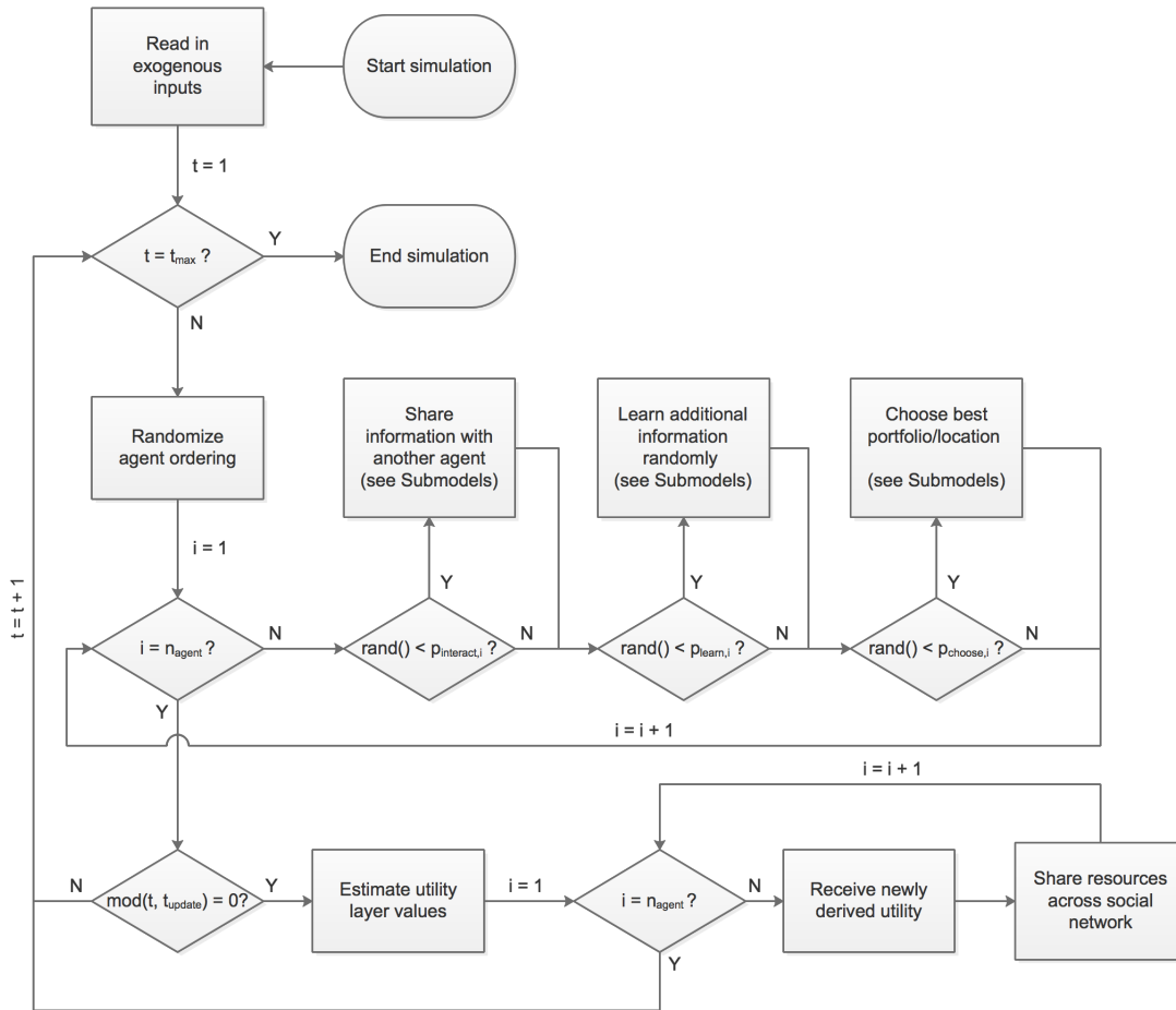
Figure 2: MIDAS process flow overview. Agent information sharing, learning, and decision flow diagrams included in Submodels section.
